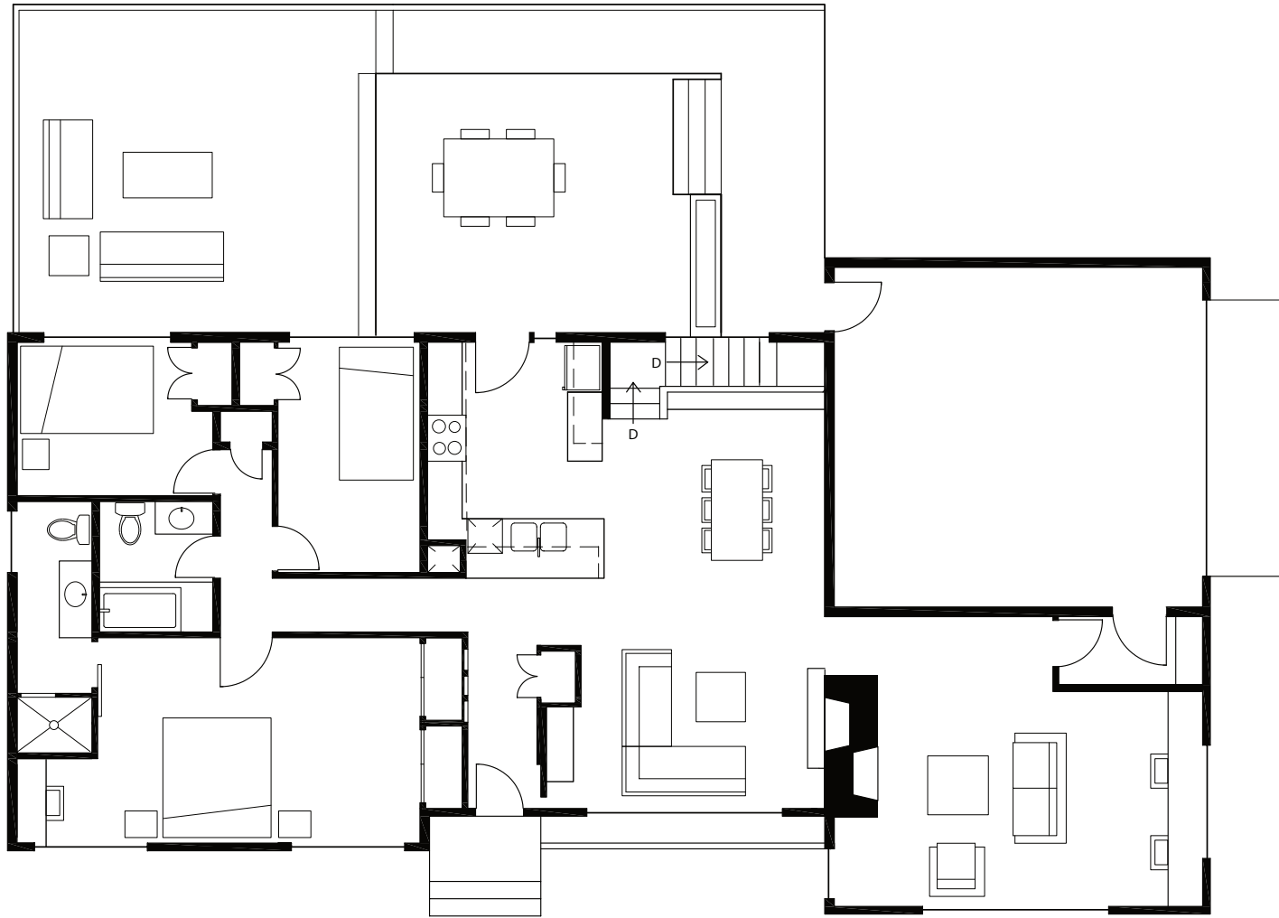
This is the final floor plan for the completed concept design, including furniture, for this week's Design Project.
