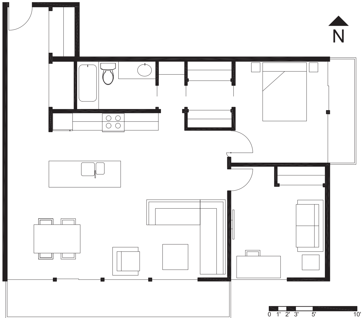
This is the final floor plan for the completed concept design, including furniture, for this week's Design Project.
